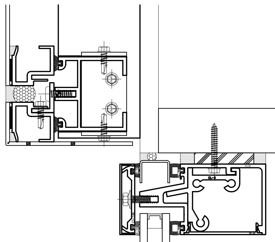
5 1 HORIZONTAL AT WINDOW HEAD FULL-DEPTH WEATHERTIGHT
