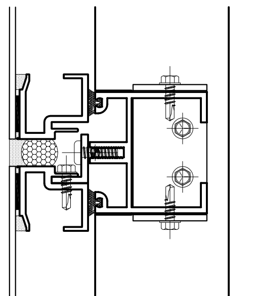
4 1 TYPICAL HORIZONTAL FULL-DEPTH WEATHERTIGHT
