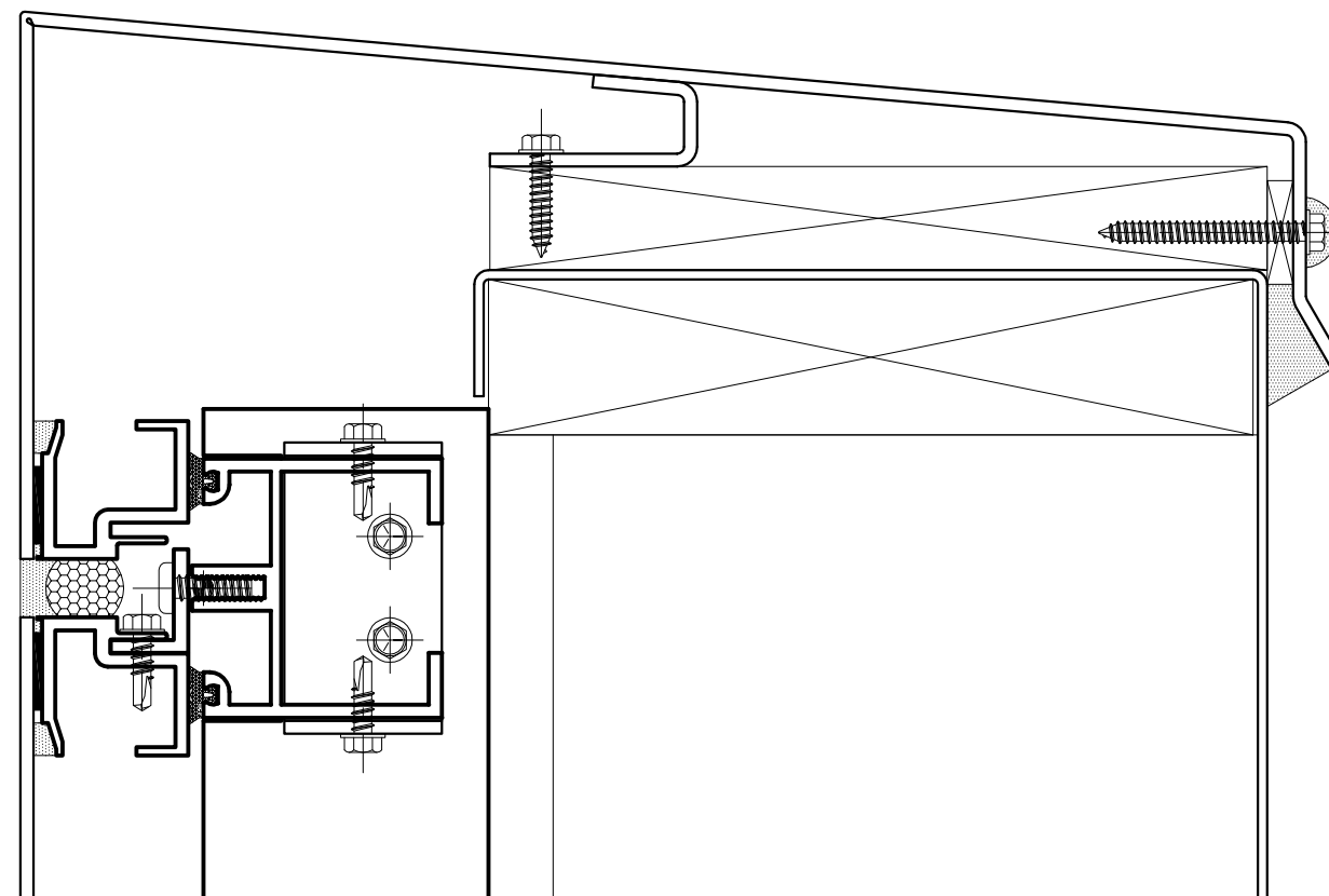
2 1 HORIZONTAL AT COPING FULL-DEPTH WEATHERTIGHT
