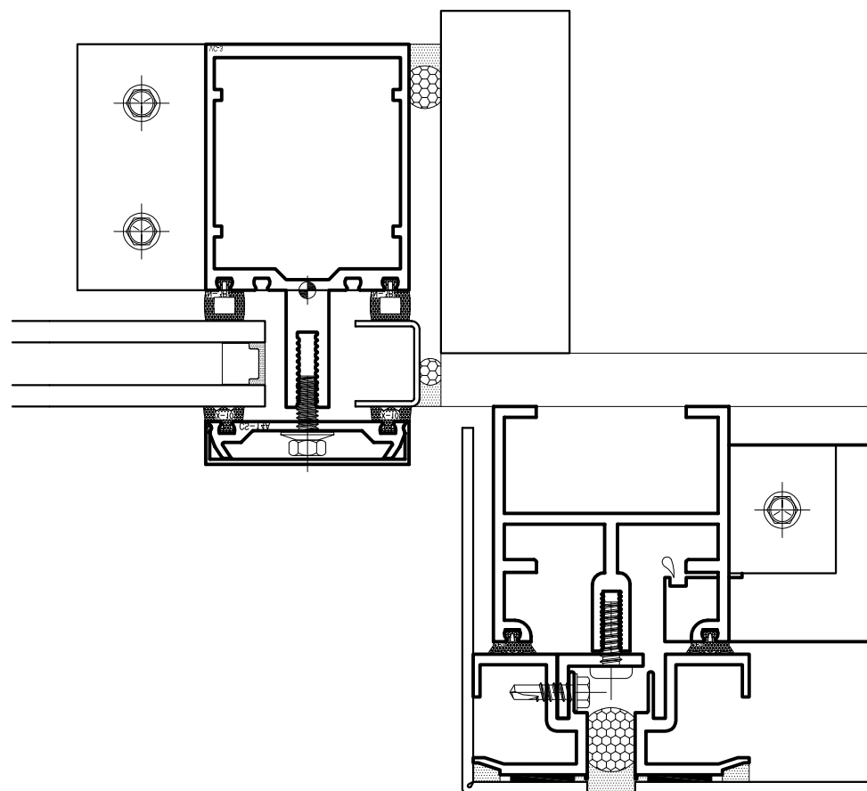
1 1 VERTICAL AT WINDOW JAMB FULL-DEPTH WEATHERTIGHT
